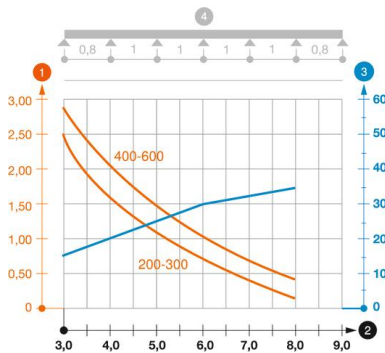
Load diagram, wide span cable tray, type WKSG 110
